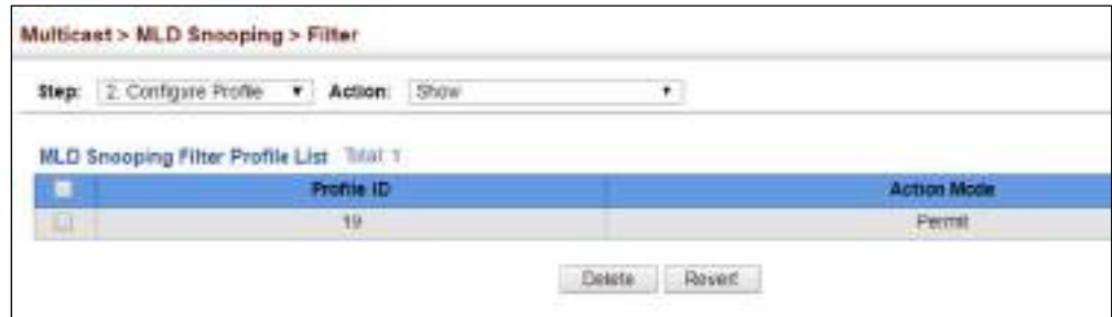
Figure 413: Showing the MLD Filtering Profiles Created
