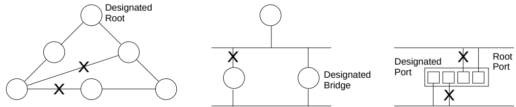
Figure 120: STP Root Ports and Designated Ports
