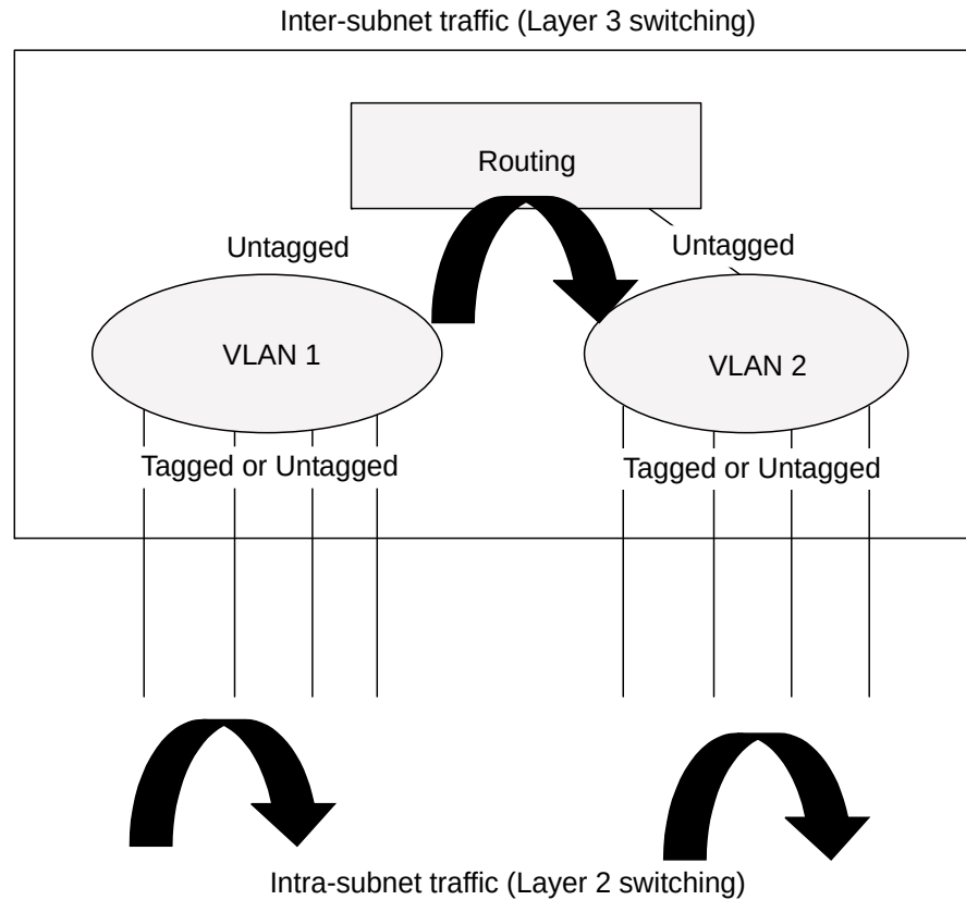
Figure 468: Virtual Interfaces and Layer 3 Routing
