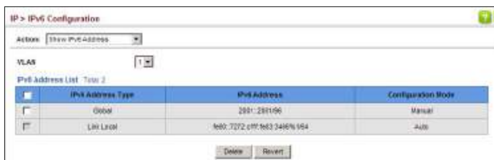
Figure 462: Showing Configured IPv6 Addresses
