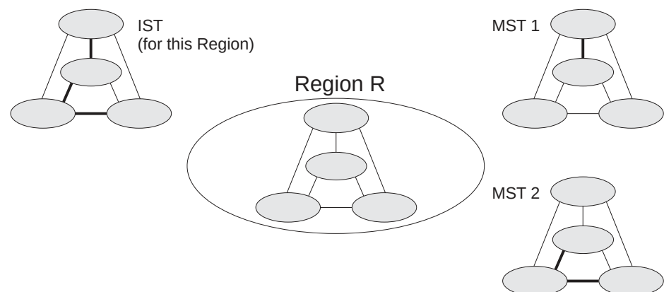
Figure 95: MSTP Region, Internal Spanning Tree, Multiple Spanning Tree
