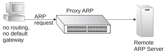
Figure 312: Proxy ARP
