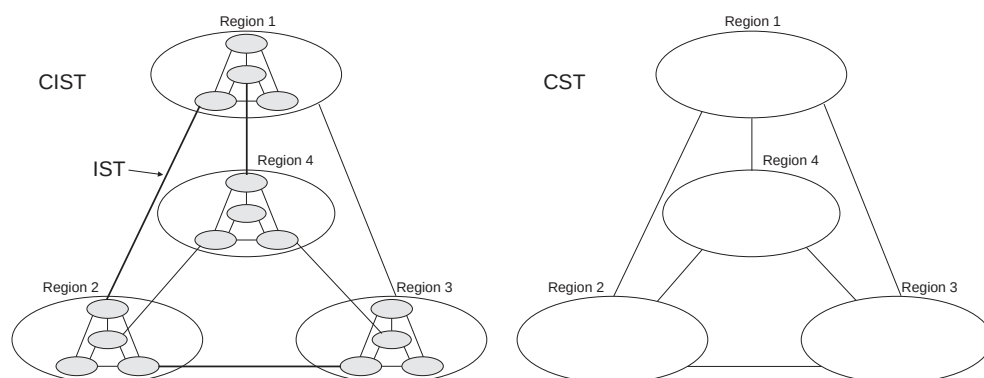
Figure 96: Spanning Tree – Common Internal, Common, Internal
