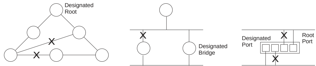
Figure 94: STP Root Ports and Designated Ports
