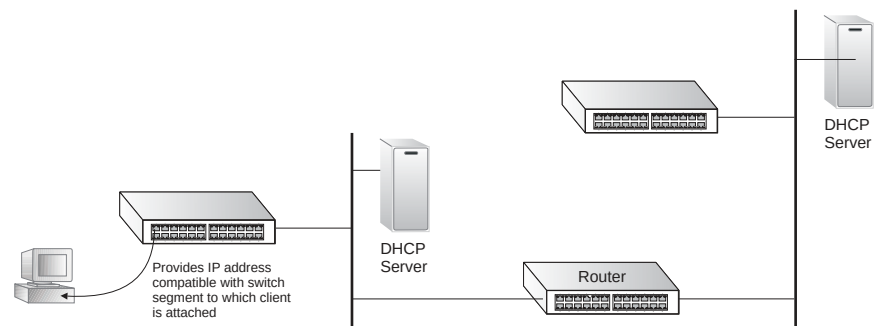
Figure 362: Layer 3 DHCP Relay Service
