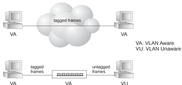
Figure 72: VLAN Compliant and VLAN Non-compliant Devices
