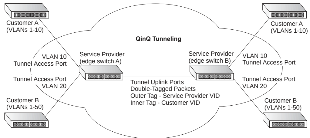
Figure 79: QinQ Operational Concept
