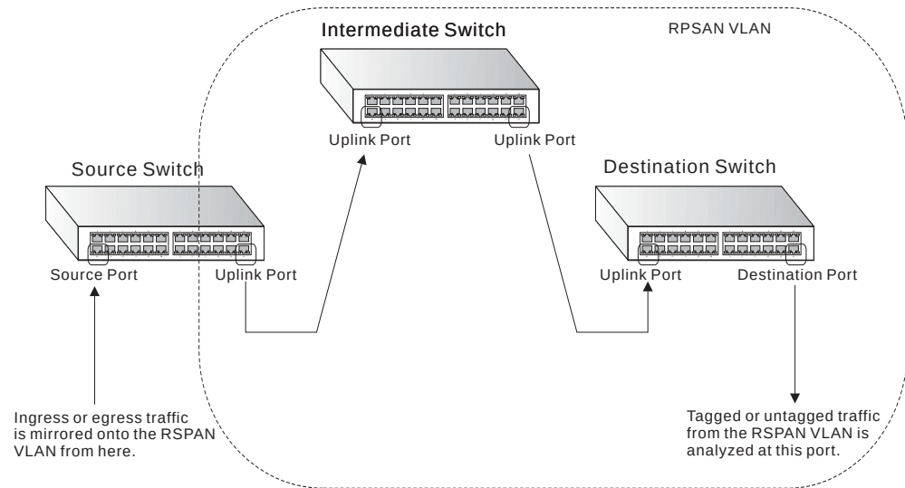
Figure 61: Configuring Remote Port Mirroring
