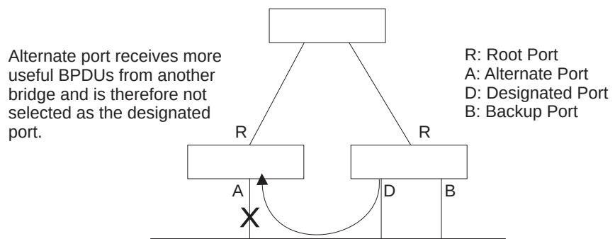
Figure 104: STA Port Roles
