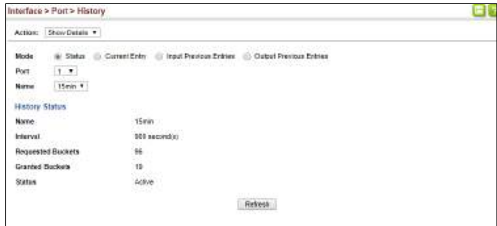
Figure 37: Showing Status of Statistical History Sample
