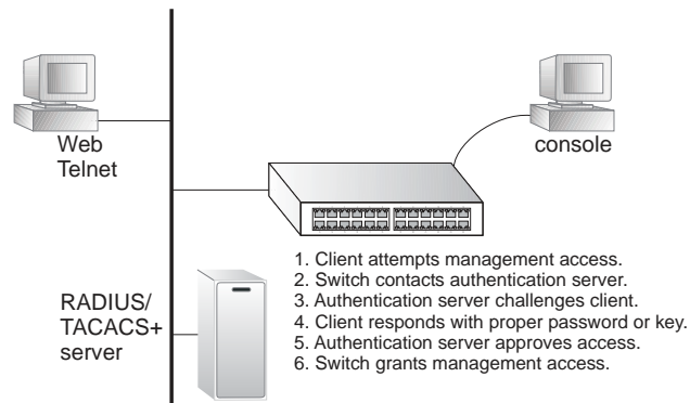
Figure 144: Authentication Server Operation
