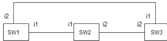
Figure 109: Determining the Root Port
