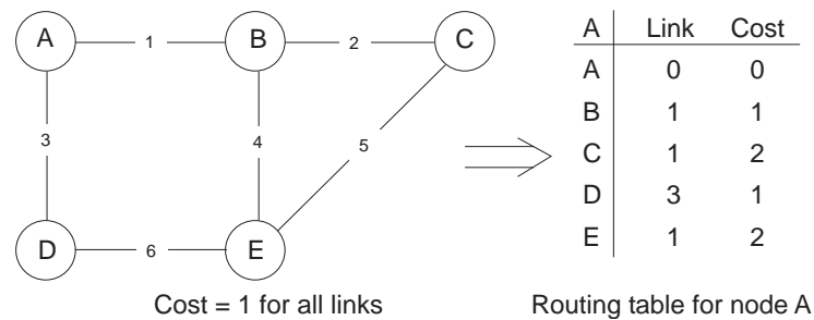
Figure 340: Configuring RIP
