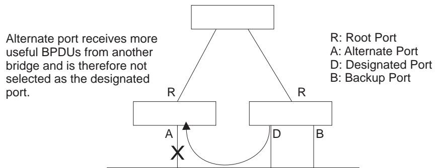
Figure 111: STA Port Roles
