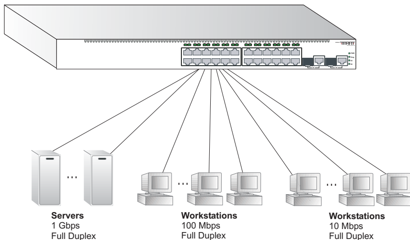
Figure 2-1 Collapsed Backbone
