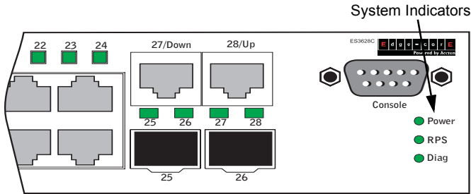
Figure 1-3 System LEDs
