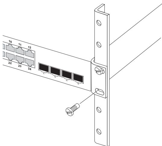
Figure 3-3 Installing the Switch in a Rack
