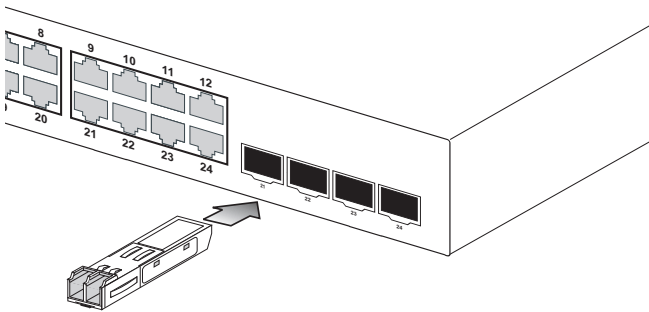
Figure 3-5 Inserting an SFP Transceiver into a Slot
