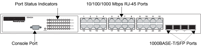
Figure 1-1 Front Panels
