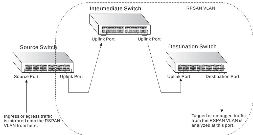
Figure 64: Configuring Remote Port Mirroring
