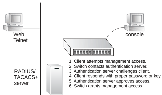
Figure 164: Authentication Server Operation
