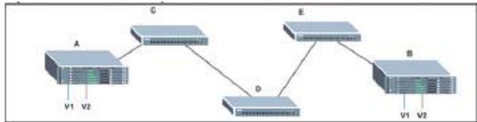
Figure 77: VLAN Trunking
