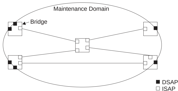
Figure 314: Single CFM Maintenance Domain
