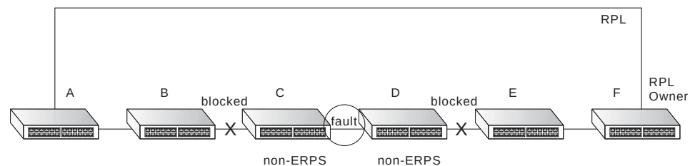
Figure 309: Non-ERPS Device Protection
