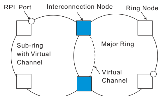
Figure 307: Sub-ring with Virtual Channel
