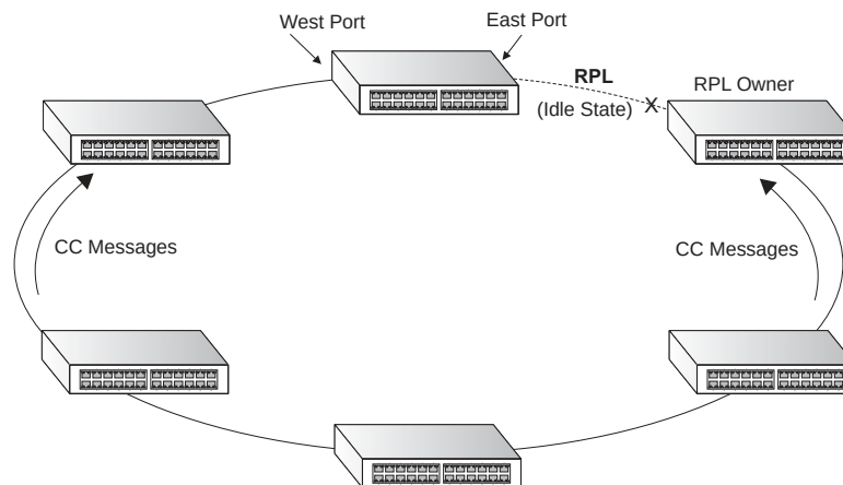
Figure 304: ERPS Ring Components
