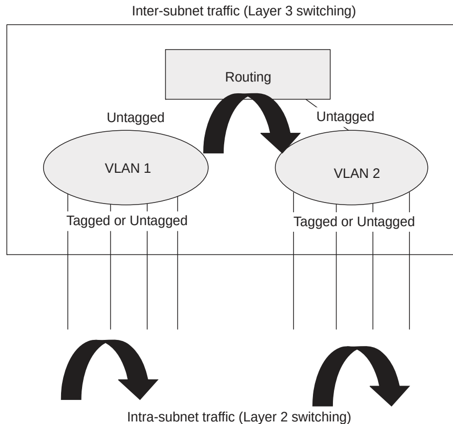
Figure 446: Virtual Interfaces and Layer 3 Routing
