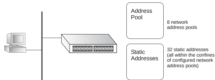
Figure 483: DHCP Server
