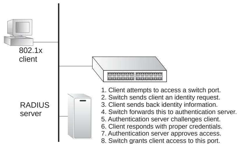
Figure 212: Configuring Port Authentication
