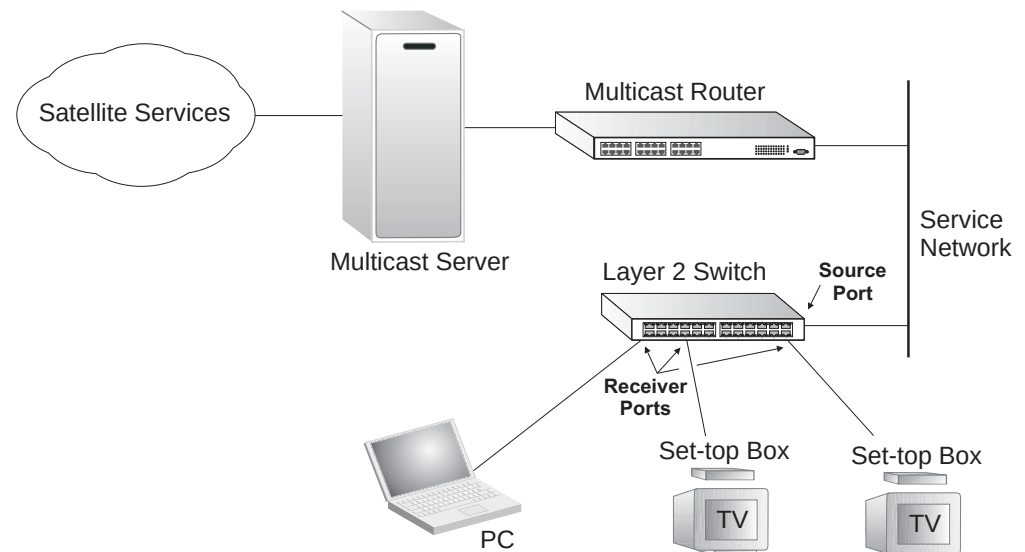
Figure 397: MVR Concept
