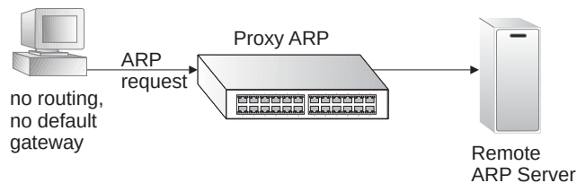
Figure 427: Proxy ARP
