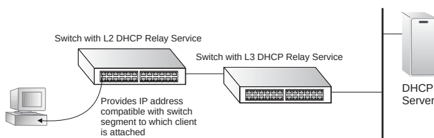
Figure 480: Layer 2 DHCP Relay Service (DHCP server on a separate network segment)
