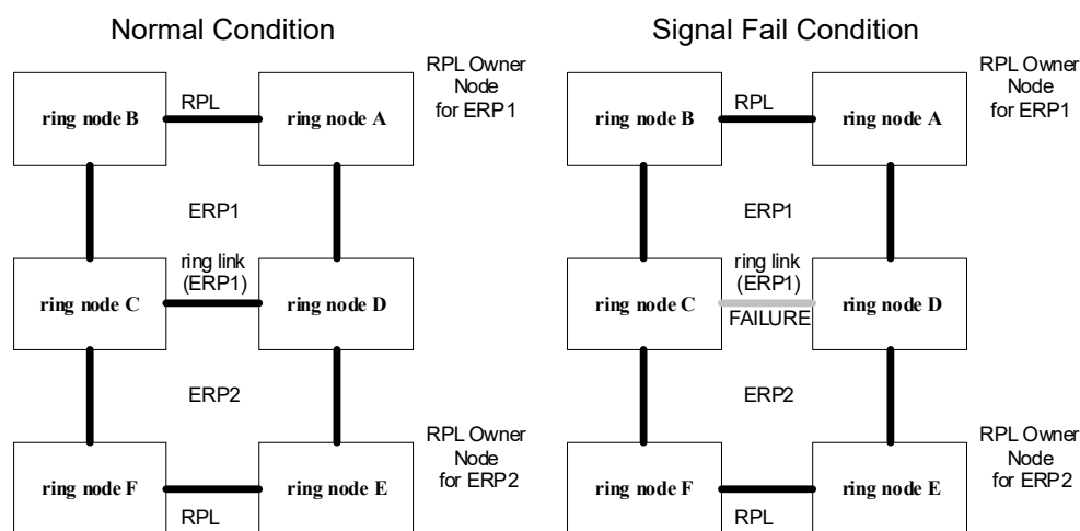
Figure 305: Ring Interconnection Architecture (Multi-ring/Ladder Network)
