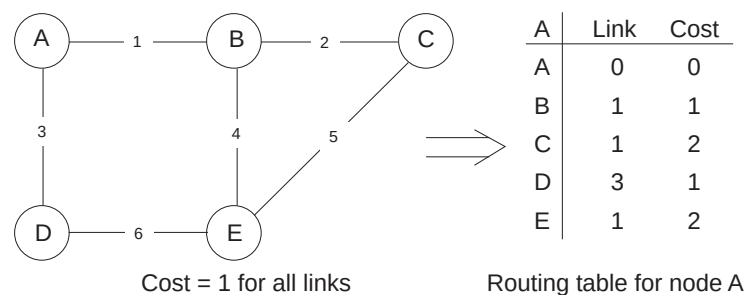
Figure 450: Configuring RIP
