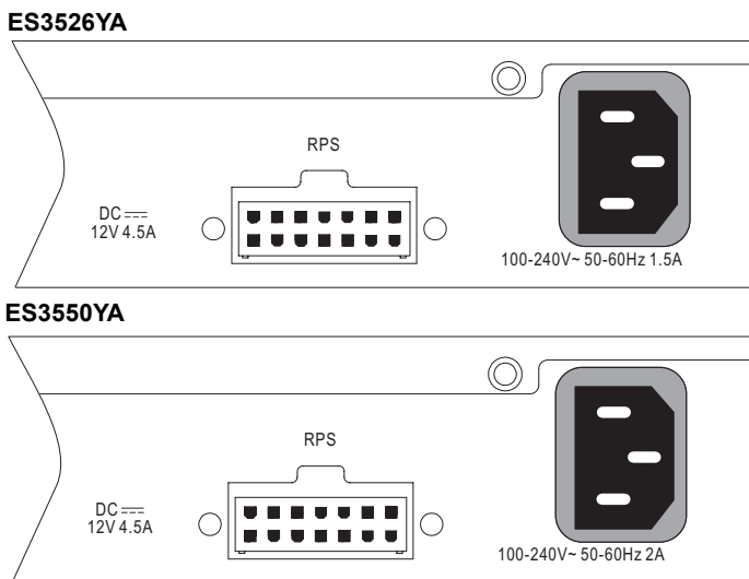
Figure 3-7 Power Receptacles
