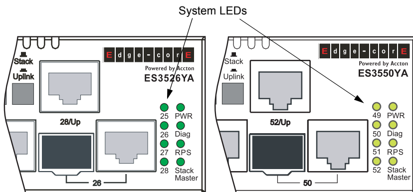
Figure 1-4 System LEDs
