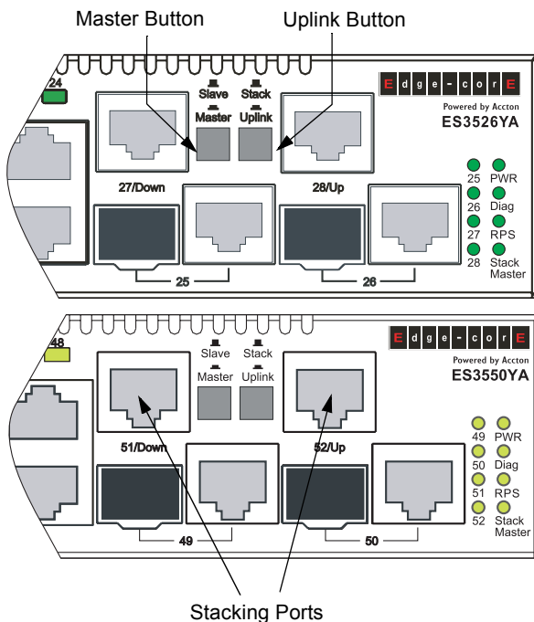
Figure 1-2 Stacking Ports
