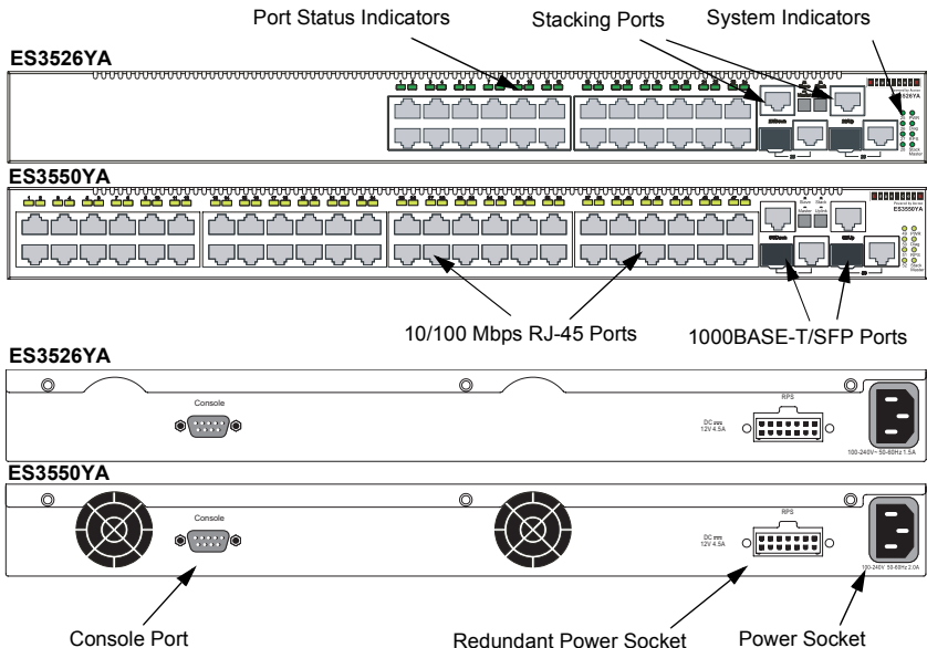
Figure 1-1 Front and Rear Panels
